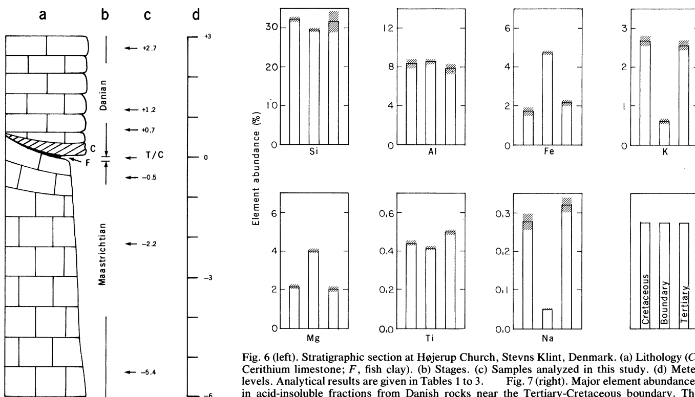
deviations for three samples. (Only two measurements of magnesium and silicon were included in the Cretaceous values.) For the boundary layer sample the crosshatched areas are the standard deviations associated with counting errors. Measurements of silicon and magnesium were done by XRF (42), all others were by NAA.
