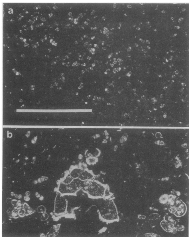
Fig. 1. Photomicrographs of (a) the basal bed of the Tertiary, showing Globigerina eugubina , and (b) the top bed of the Cretaceous, in which the largest foraminifer is Globotruncana contusa . Both sections are from the Bottaccione section at Gubbio; they are shown at the same scale and the bar in (a) is 1 mm long.
